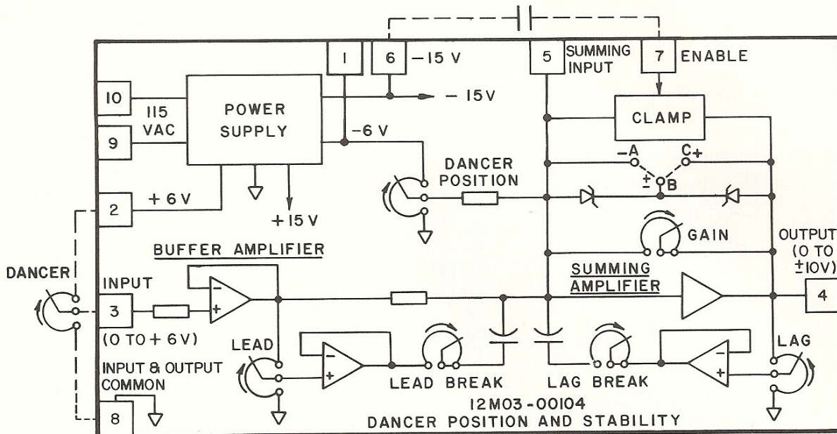
FIGURE 1 SIMPLIFIED SCHEMATIC
